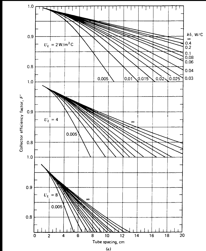
Figure 6.5.4 Collector efficiency factor F' versus tube spacing for 10 mm diameter tubes: (a) k_{\bar{r}} = 100 \text{ W/m}^2 \text{ C} ; (b) h_{fi} = 300 \text{ W/m}^2 \text{ C} ; (c) h_{fi} = 1000 \text{ W/m}^2 \text{ C}
