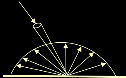
Diffuse reflection
