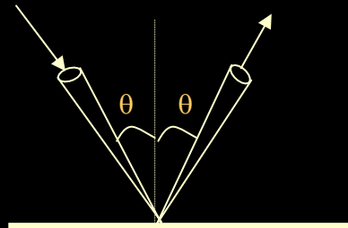
Specular reflection
