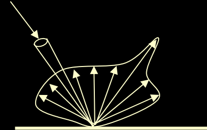
General reflection
